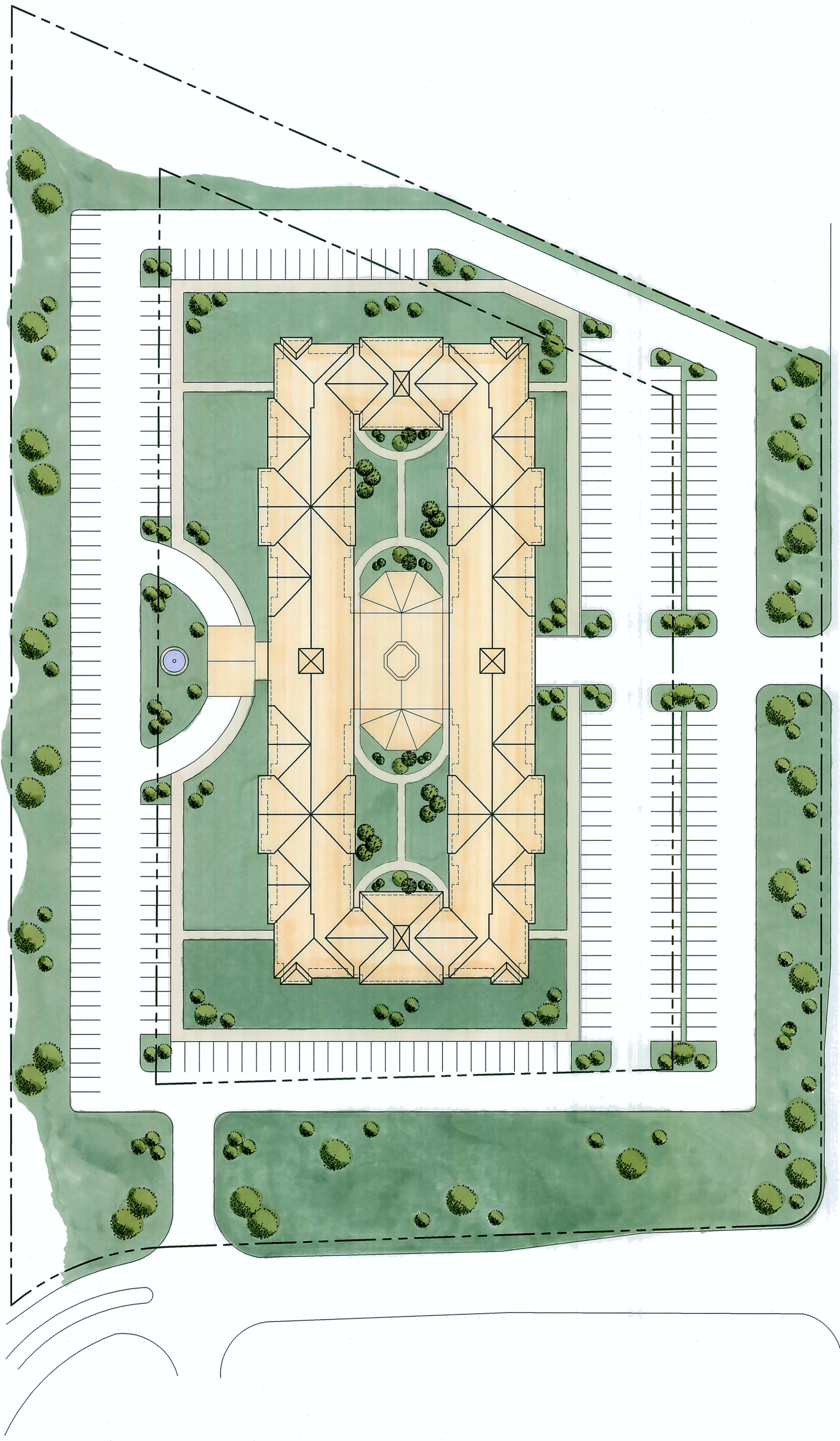
Schematic Site Plan 1" = 40' 0" TOTAL PARKING SPACES: 280
